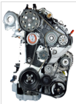
Timing Drive System
